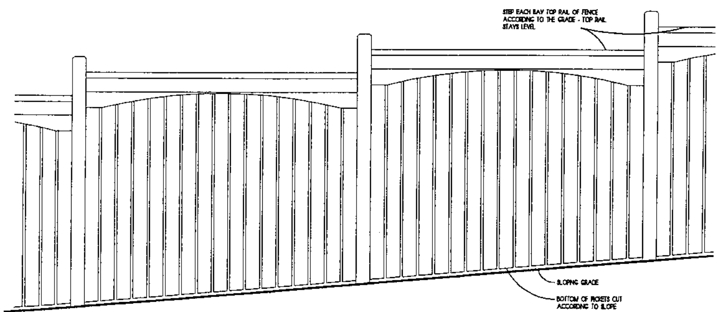
2 A12 FENCES FACING STREETS AND OPEN AREAS FENCE DETAILS NYS
