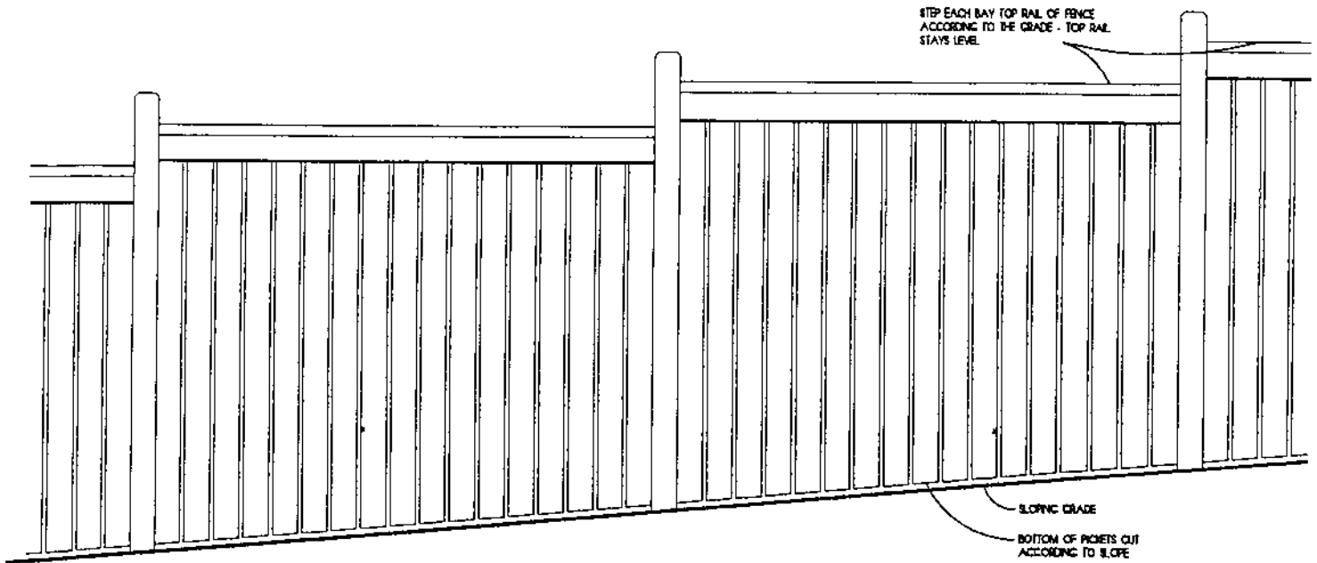
1 A12 FENCES FACING INDIVIDUAL LOTS FENCE DETAILS NYS
